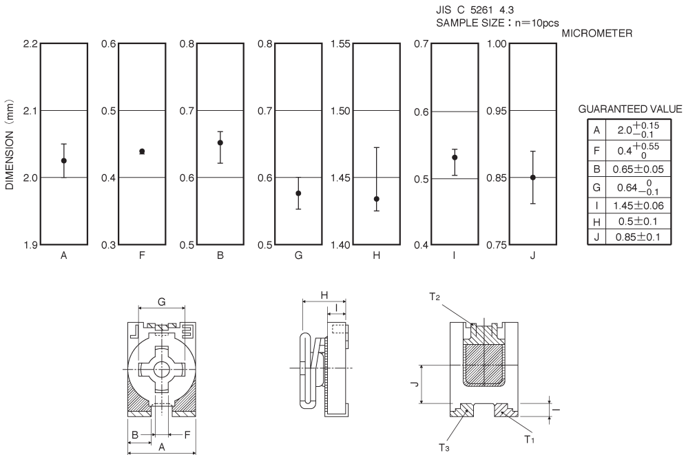
Fig.2 Dimensions
