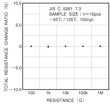
Fig.10-1 Temperature cycling
