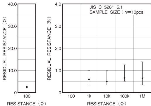
Fig.4 Residual resistance
