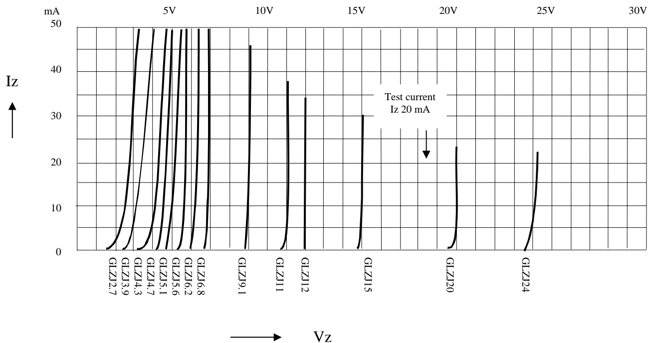
FIG.1- BREAKDOWN CHARACTERISTICS
