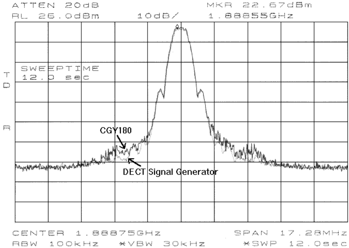
Spectrum of amplified DECT signal
