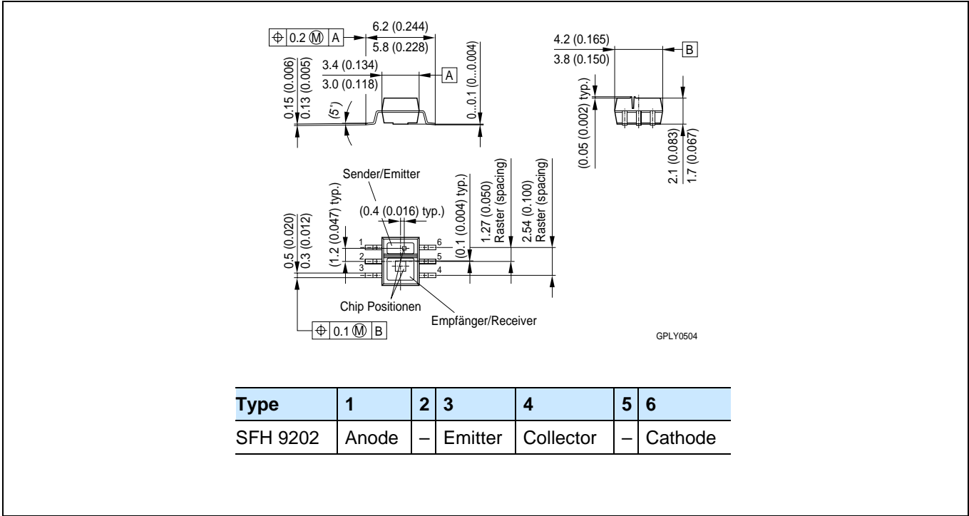
Maße in mm (inch) / Dimensions in mm (inch).
