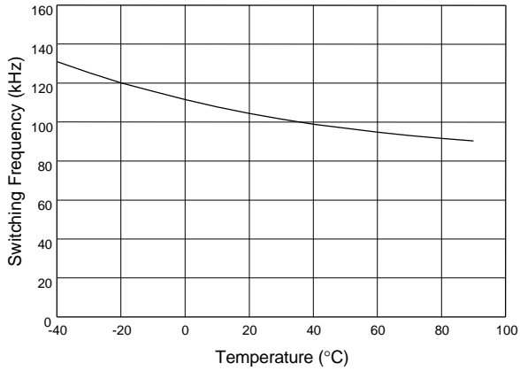
Fig. 13 AIC1642-30 Switching Frequency vs. Temperature
