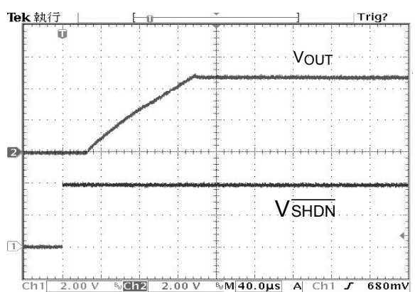
Fig. 18 Start-Up Time
