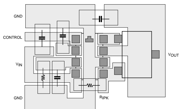
SOT-23L-8 BOARD LAYOUT
