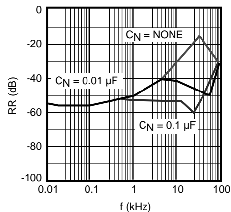
RIPPLE REJECTION
