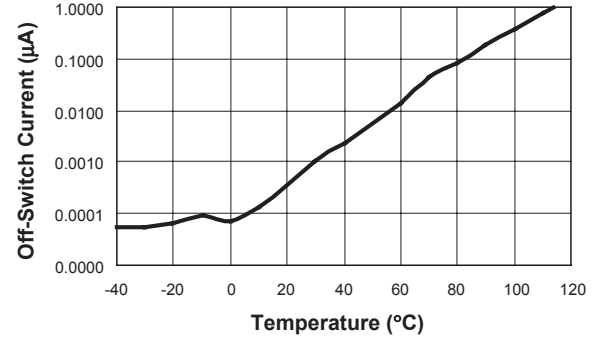
Off-Switch Current vs. Temperature
