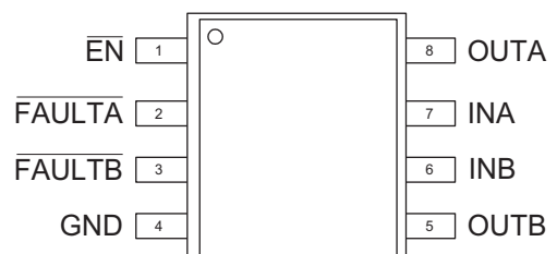
MSOP-8
