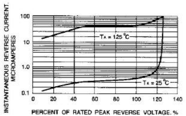
Fig. 4-TYPICAL REVERSE CHARACTERISTICS
