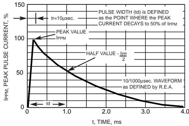
FIG. 3 - PULSE WAVEFORM
