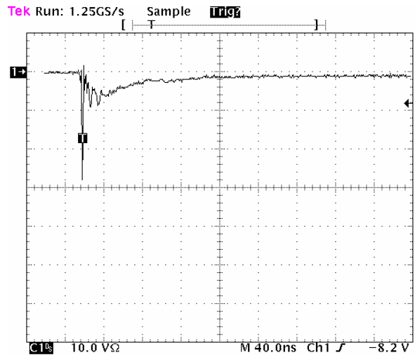
Figure 5. Negative 8 kV contact per IEC 61000-4-2 - ESD9X5.0ST5G
