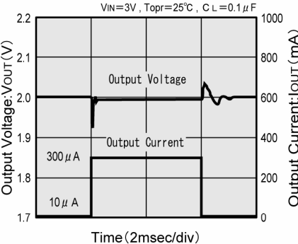
XC62RP2002 (2V)
