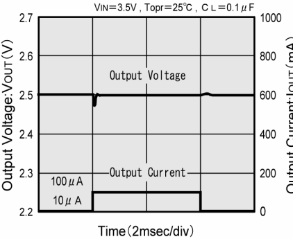
XC62RP2502 (2.5V)
