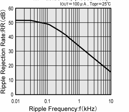
XC62RP2502 (2.5V)
