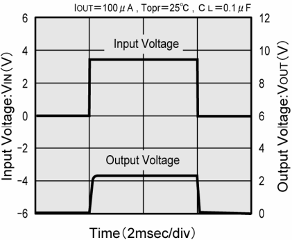
XC62RP2502 (2.5V)
