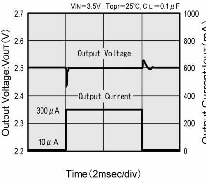
XC62RP2502 (2.5V)
