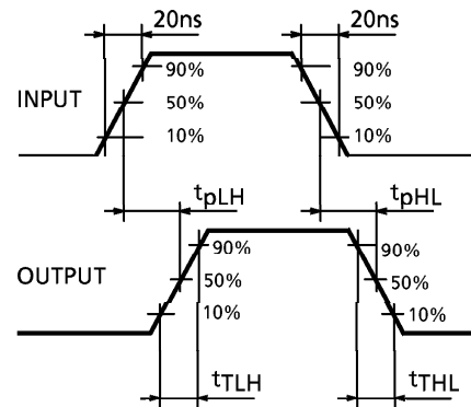
WAVEFORM
