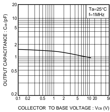
Fig.8 Back capacitance voltage
