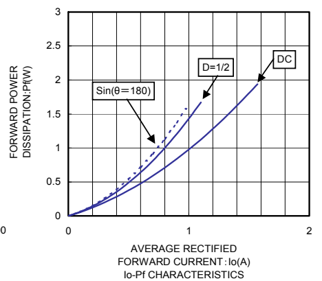
I_{o-PF} CHARACTERISTICS
