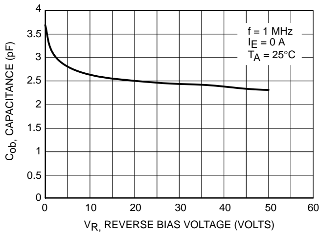
Figure 29. Output Capacitance
