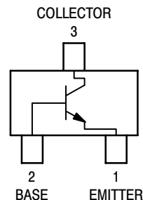
CASE 318D-04, STYLE 1 SC-59
