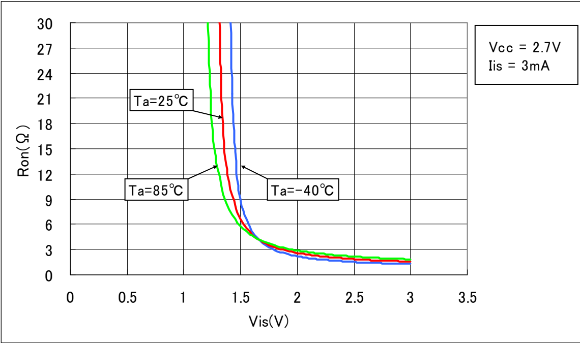
R ON -V IN Characteristic Curves V CC = 2.7 V, I is = 3 mA, T a = -40/25/85°C
