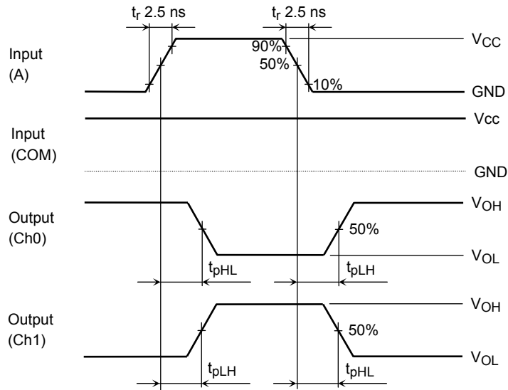
Figure 2 t_{pLH} t_{pHL}
