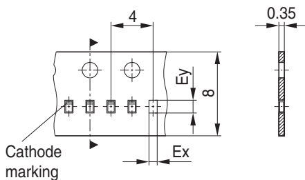
Figure 15 PG-TSSLP-2-2: Packing
