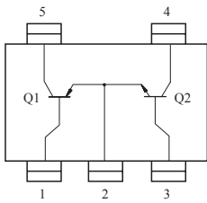
EQUIVALENT CIRCUIT(TOP VIEW)
